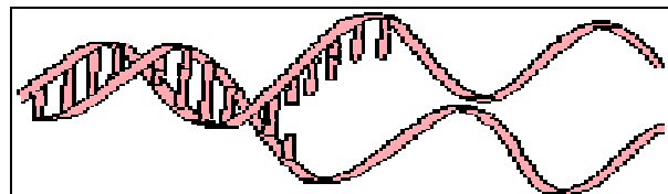
DNA Strand
